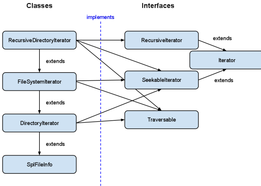
Figure B.1. SPL's classes and interfaces
